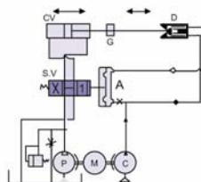
Circuit Component
