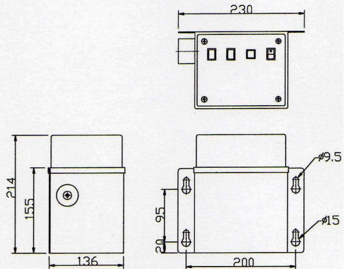
High-Voltage ion generator (9kg)
