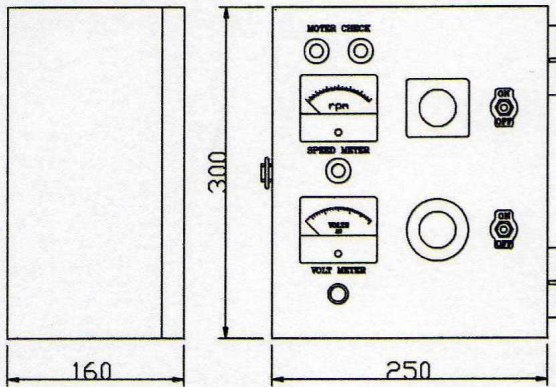
Control Box (10kg)
